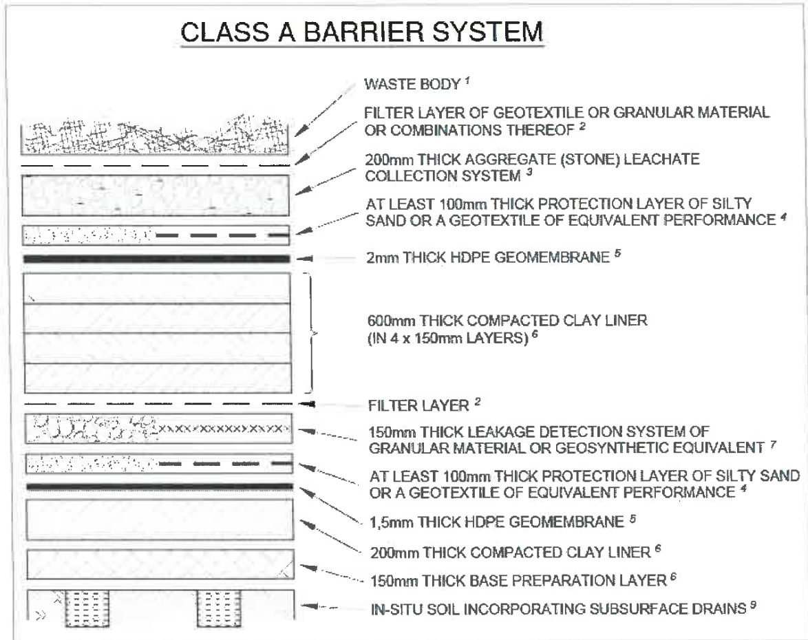
(a) Class A Barrier System
