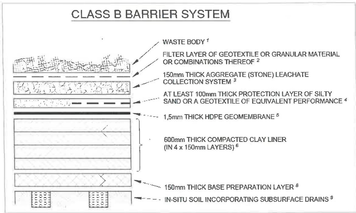
(b) Class B Barrier System
