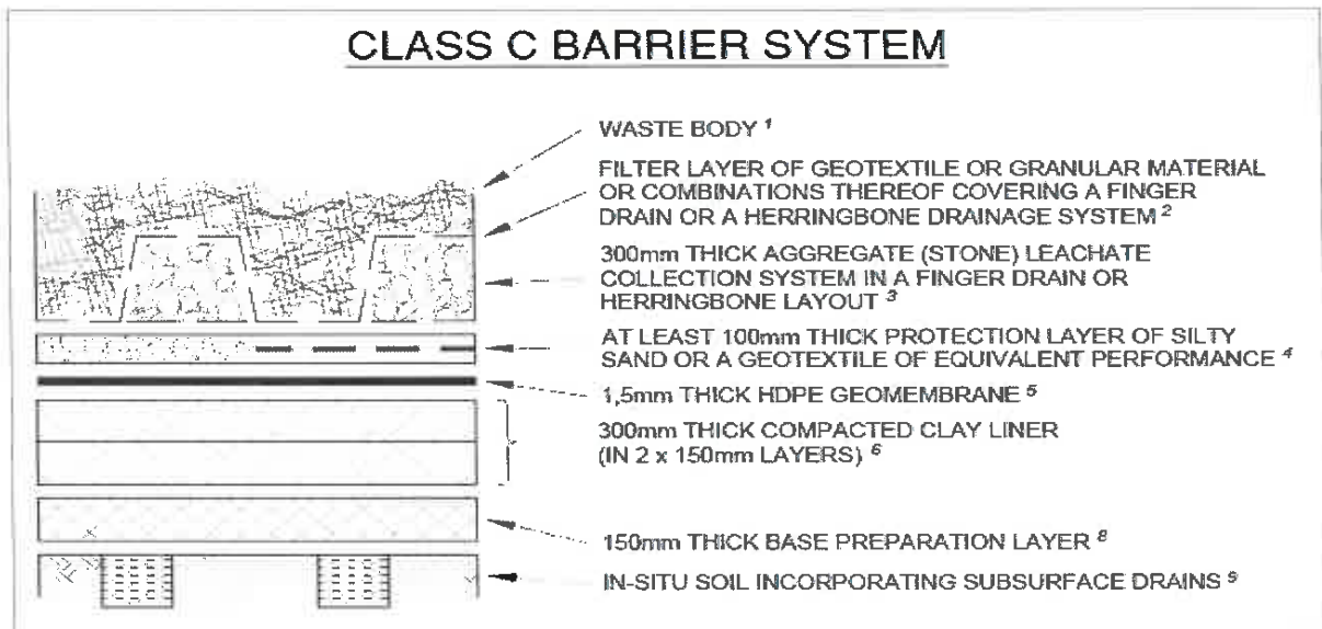
(c) Class C Barrier System
