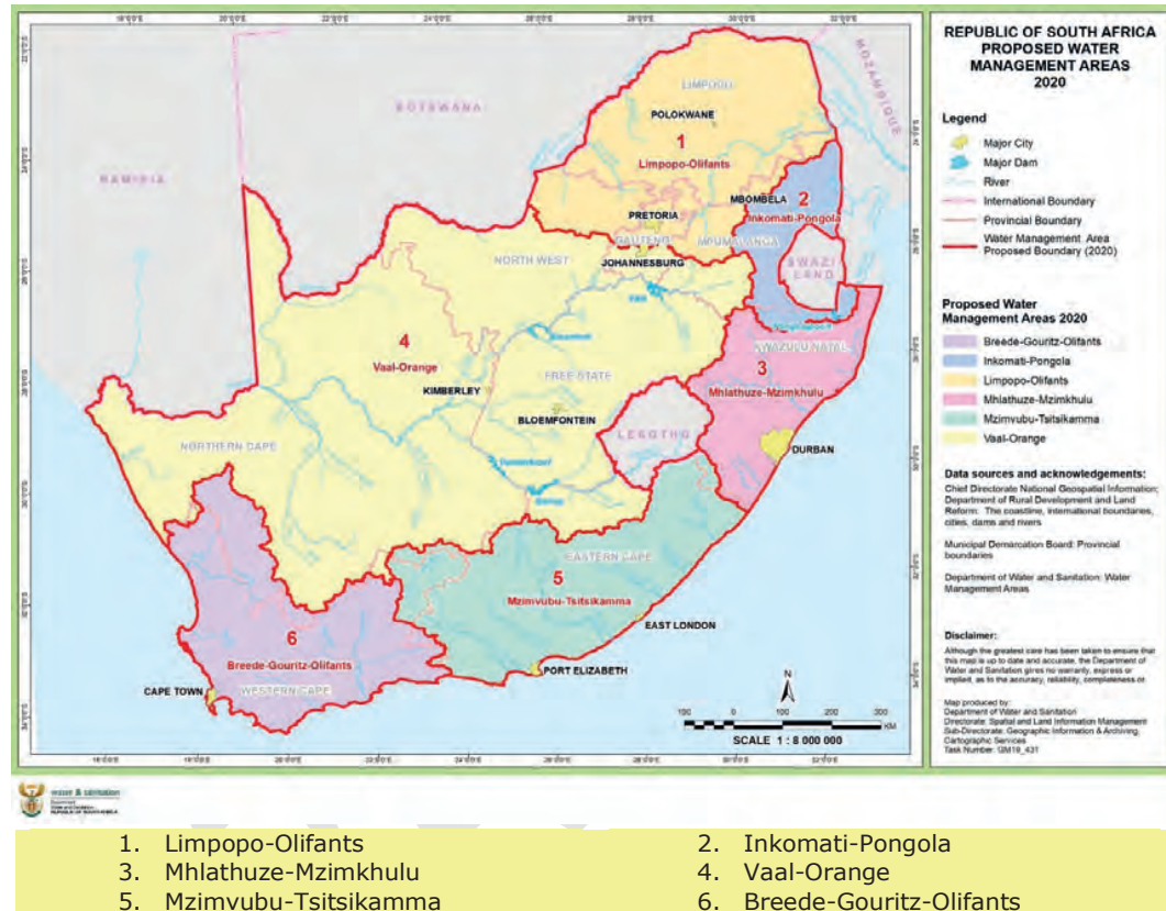
Figure 4: Proposed Water Management Areas within South Africa
