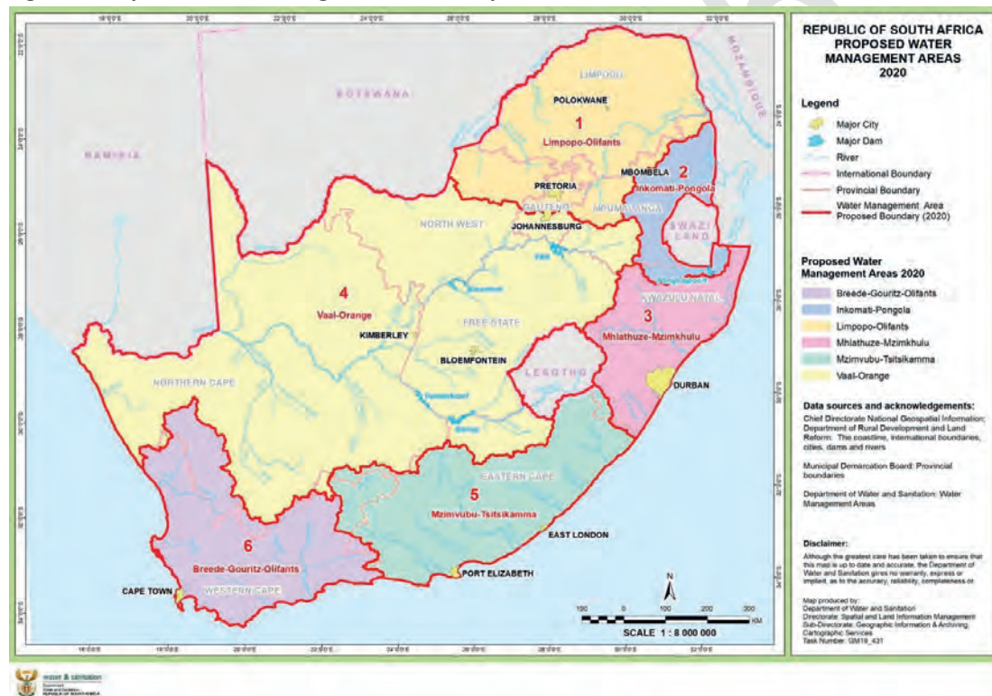
Figure 1: Proposed Water Management Areas Map
