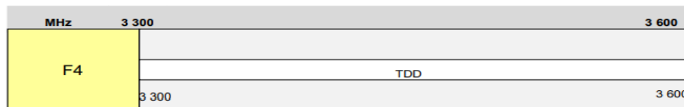
Figure 15: Frequency arrangements, 3300 – 3600 MHz 114
