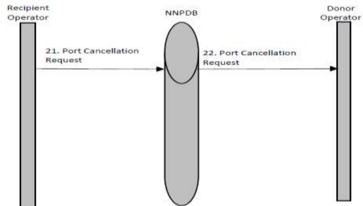
Figure 3: Port Cancellations"
